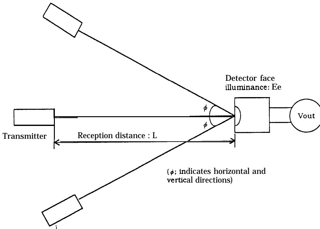
Fig.2 Standard optical system
